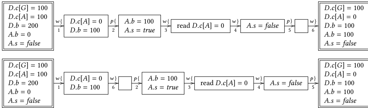
Fig. 5. Two traces of calls illustrating the original and callback-free versions of a failed attack on the ECF version of the DAO. Nodes are labeled by local changed states and edges are labeled by actions and by the corresponding order in the original trace. D denotes the DAO, G denotes a GoodClient and A is an Attacker object. w denotes the withdrawAll operation and p denotes the pay operation. b is a shorthand for balance, c is a shorthand for credit, and s is a shorthand for stop.
