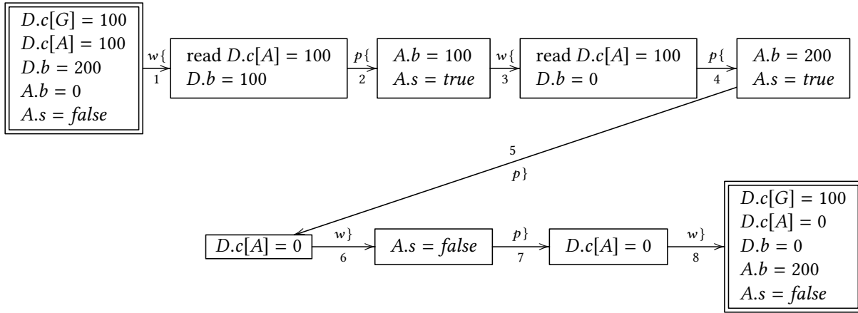
Fig. 4. A trace of calls illustrating an attack on the DAO. Nodes are labeled by local changed states and edges are labeled by actions and by the corresponding order in the original trace. D denotes the DAO, G denotes a GoodClient and A is an Attacker object. w denotes the withdrawAll operation and p denotes the pay operation. b is a shorthand for balance, c is a shorthand for credit, and s is a shorthand for stop.
