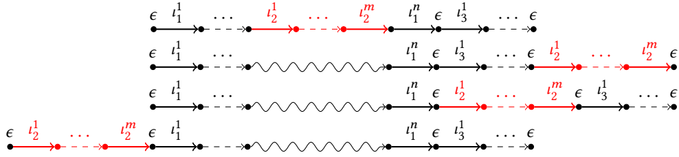
Fig. 9. The callback reorder process. The first graph represents the original execution, which contains a callback (in red). The three other graphs represent all possible callback free executions. Red marks the moved callback transitions. Wave edges indicate that a call was replaced with a havoc transition.
