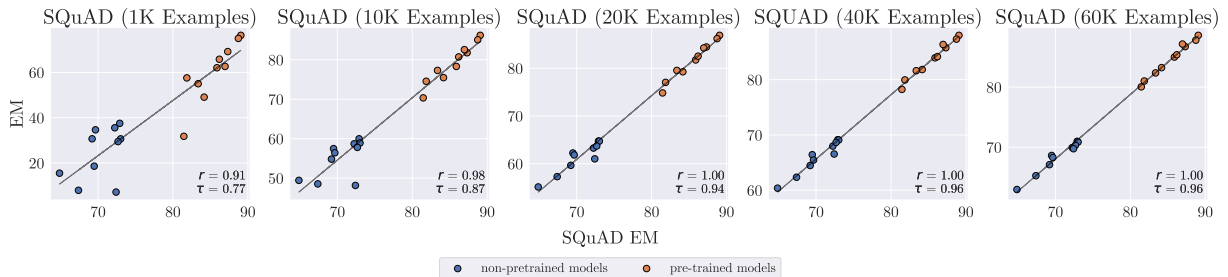
Figure 3: Downsampling the SQuAD training dataset can yield high concurrence with the full SQuAD benchmark on both pre-trained and non-pre-trained models. In particular, 10K training examples are sufficient for high concurrence on pre-trained models, and 20K examples yields high concurrence on non-pretrained models.
