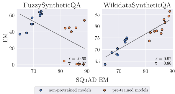
Figure 7: Left: FuzzySyntheticQA has high concurrence with SQuAD on non-pre-trained modeling approaches, but pre-training does not increase performance, leading to low overall concurrence. Right: Despite lacking natural language structure, WikidataSyntheticQA has high concurrence with SQuAD.
