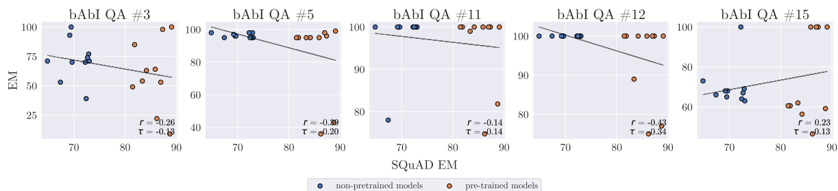
Figure 5: Modeling approaches perform perfectly or at near-chance performance on the bAbI tasks, limiting their ability to recapitulate historical findings on SQuAD (representative subset of results pictured, see Appendix D.3 for the full results on all tasks).
