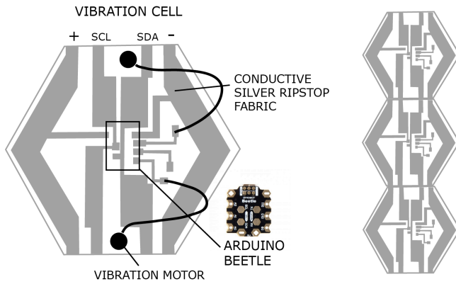
Figure 3. Circuit diagram for vibration and chain of cells
