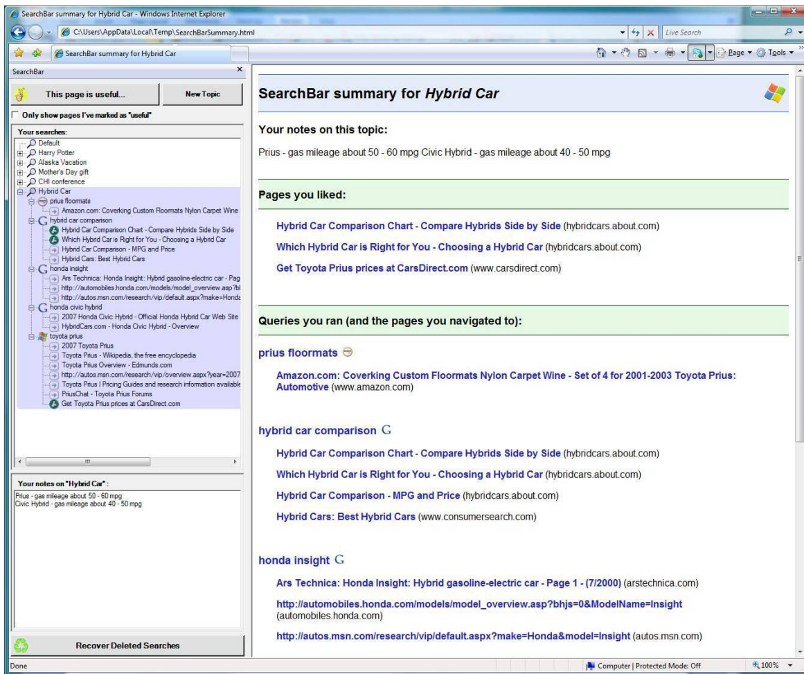
Figure 1: A screenshot showing SearchBar running within Internet Explorer. The SearchBar (left pane) includes a hierarchical history of recent search topics, queries, and results visited, along with the user’s notes on the current topic. The right pane is a standard Web browser, currently showing a summary of the active SearchBar topic.
