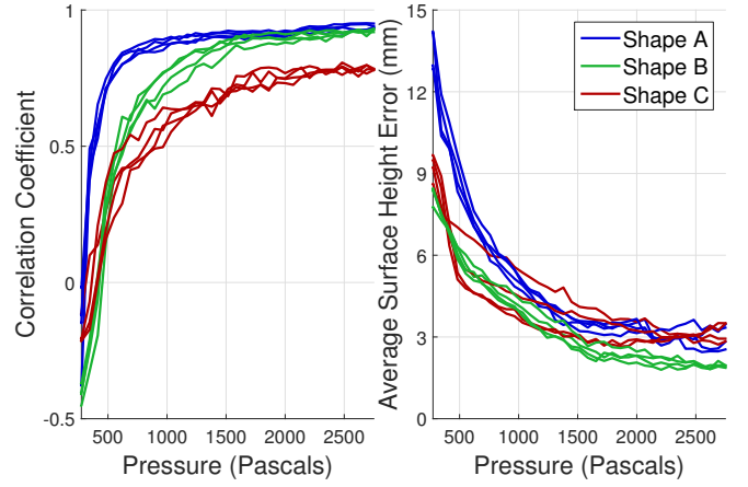
Fig. 5. As the shape control algorithm incrementally increases chamber pressure and jams cells or pins nodes when they reach their respective desired curvature or height, the correlation between the desired input shape and the output shape increases and the average height error across the surface decreases.
