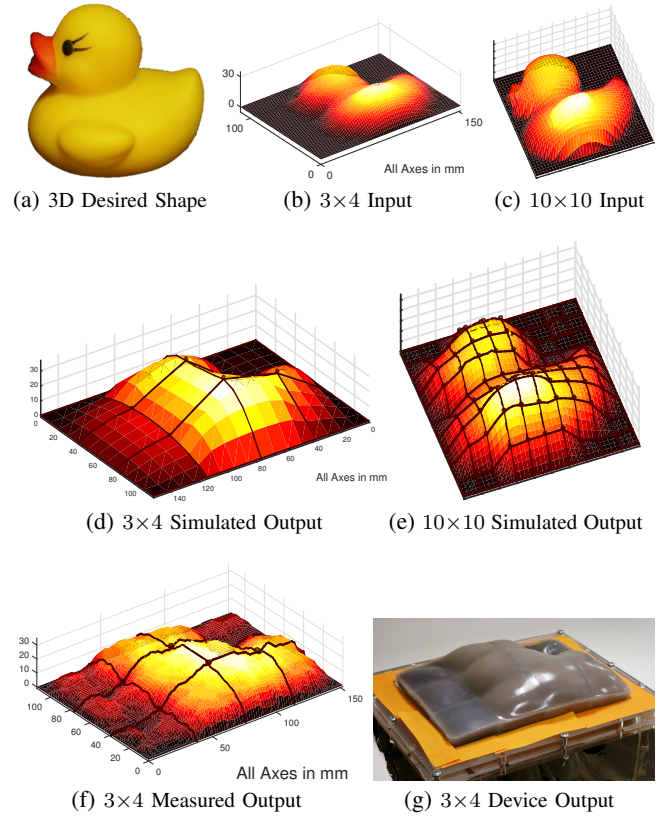
Fig. 6. A Haptic Jamming surface can render various 3D objects, like a duck (a), by z-buffering an image to convert to a desired shape input for a 12-cell array (b) or 100-cell array (c). While the simulated output shape (d) and actual output from a 3 \times 4 -cell array prototype (g) results in limited output correlation (f) to the input, a simulation of a 10 \times 10 -cell array promises more compelling outputs from larger arrays (e).
