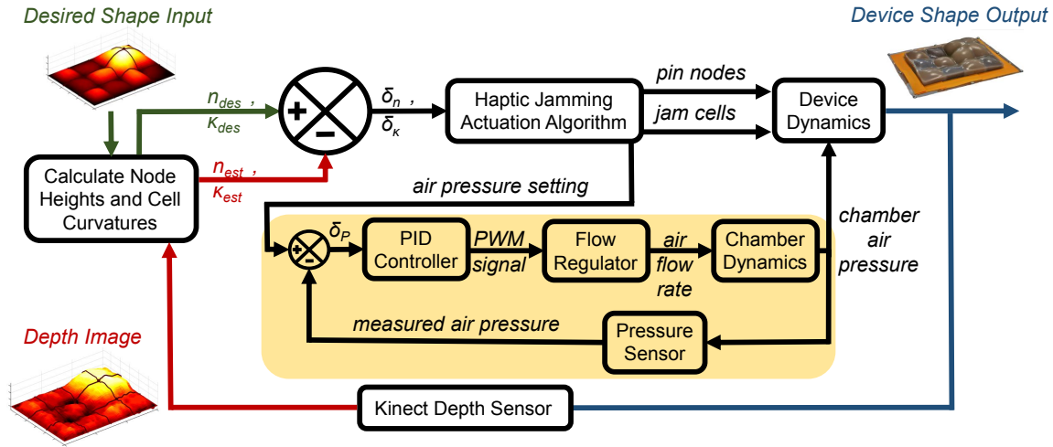
Fig. 3. A block diagram of the system control architecture. The outer loop runs once per iteration of Algorithm 1 while the inner pressure control loop, highlighted in yellow, runs continuously.
