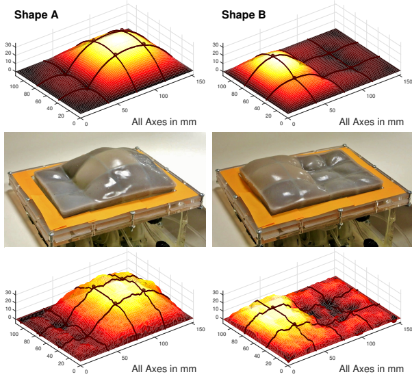
Fig. 4. Two of the desired input shapes (top) used to evaluate the system, their corresponding outputs on a 12-cell array (middle), and their surface shape measurements from the depth camera (bottom).
