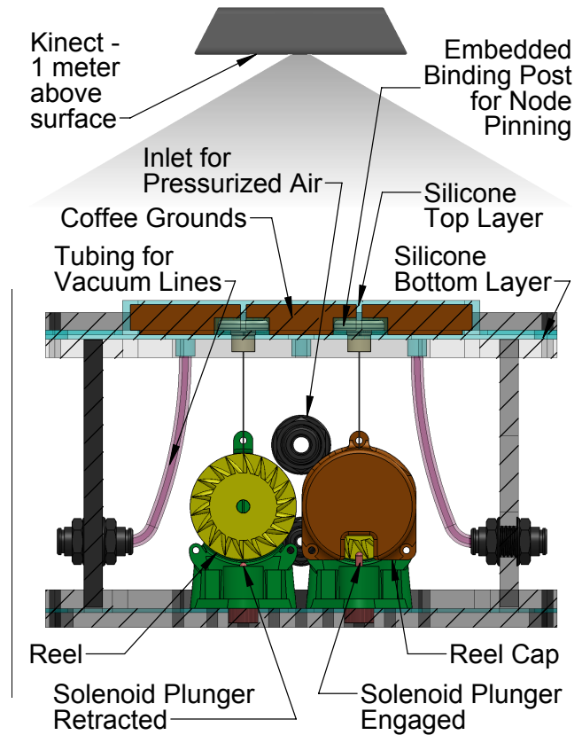
Fig. 2. A cross section of the 12-cell Haptic Jamming device shows one column of cells and nodes with the underlying mechanisms for cell jamming, node pinning, and chamber pressurization.
