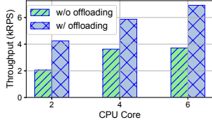
Figure 27: Throughput improvement with offloading.
