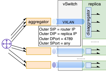
Figure 9: Session aggregation and disaggregation.
