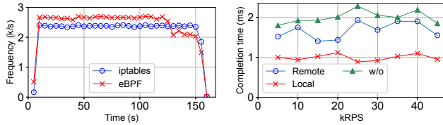
Figure 22: Higher context switch frequency of eBPF (16B packets, 4kRPS).
