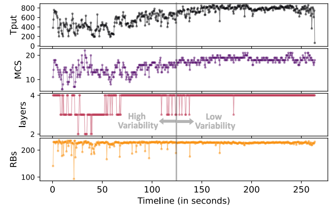
Figure 13: Impact of 5G parameter variability on 5G throughput ( V_{Sp} ) [4.4mins - 264 Seconds traces]. [ t=60 ms.]
