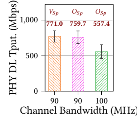
Figure 2: DL Tput. with CQI \geq 12 for Vodafone & Orange Spain with 90 MHz, and Orange Spain with 100 MHz.
