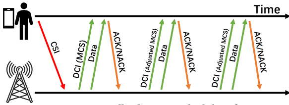
Figure 21: CSI Feedback & DCI scheduling for DL.
