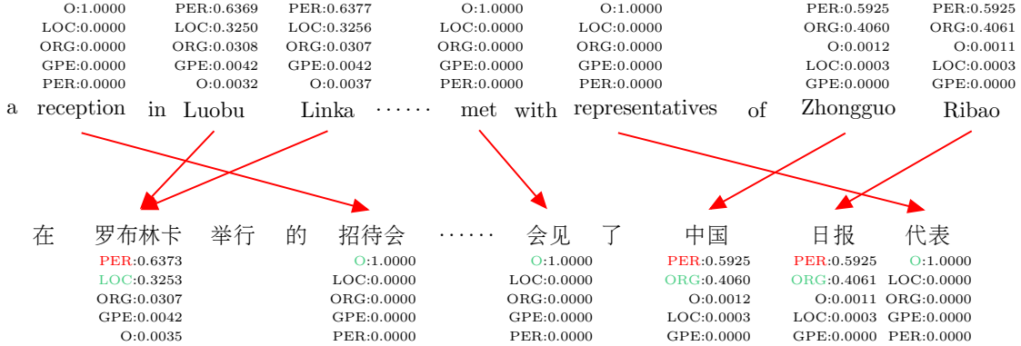
Figure 1: Diagram illustrating the projection of model expectation from English to Chinese. The posterior probabilities assigned by the English CRF model is shown above each English word; automatically induced word alignments are shown in red; the correct projected labels for Chinese words are shown in green, and incorrect labels are shown in red.
