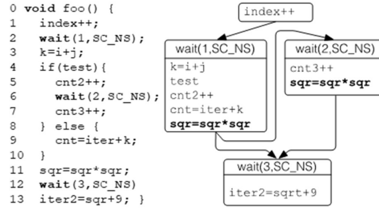
Figure 3: Example SystemC Code and corresponding Segment Graph [13]
