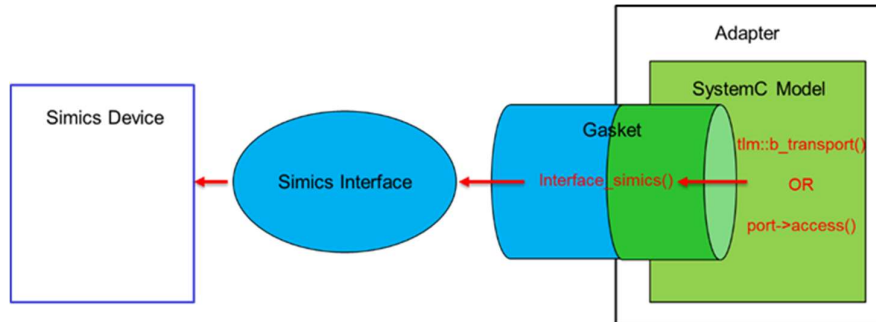
Figure 7: SystemC-to-Simics communication
