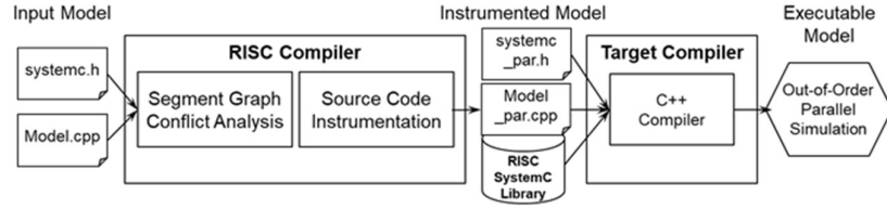
Figure 2: RISC Compiler and Simulator Flow [14]
