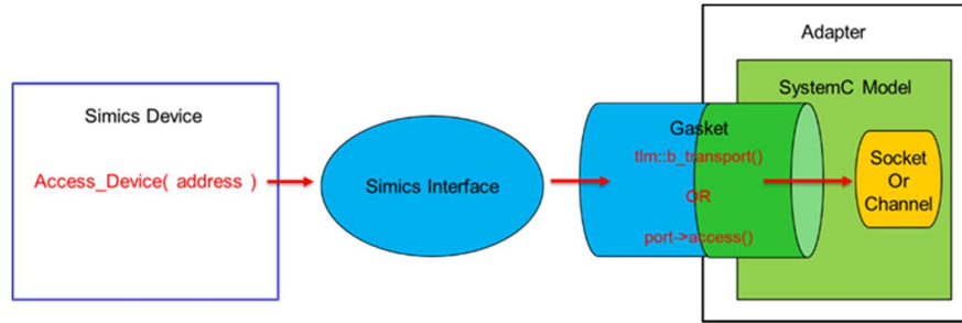
Figure 6: Simics-to-SystemC communication
