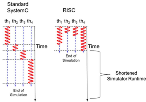
Figure 1: Juxtaposition between standard SystemC and RISC thread activity over time.
