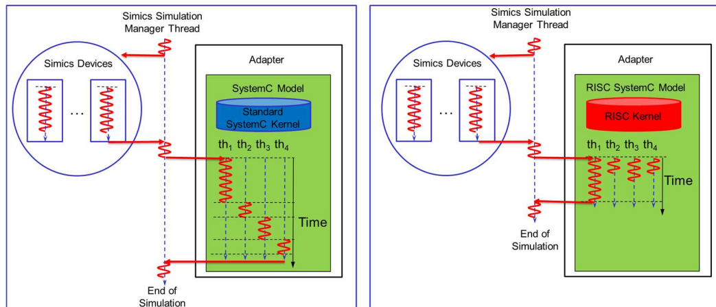
Figure 5: Two different Simics simulations of the same model with the left-side using a standard SystemC kernel and the right-side featuring RISC kernel for out-of-order parallel multithreading of SystemC threads
