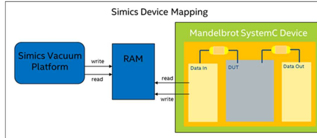
Figure 9: Simics Device set up for Mandelbrot Renderer example
