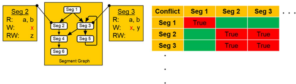
Figure 4: Segment Graph Based Conflict Analysis [8]
