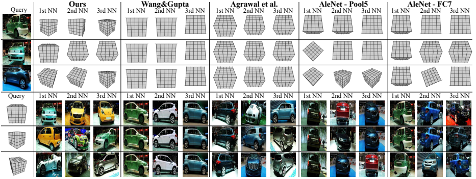
Fig. 8: NN search results between EPFL dataset images and a synthetic cube defining an abstract 3D pose. See the supplementary material (section 5) for tSNE embedding of all cubes and car poses in a joint space. Note that the 3D poses defined by the cubes are 90° congruent.
