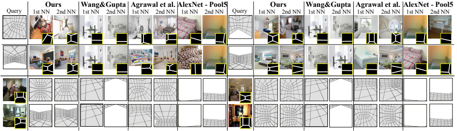
Fig. 7: Scene layout NN search results between LSUN images and synthetic concave cubes defining abstract 3D layouts. Images with yellow boundary show the ground truth layout.
