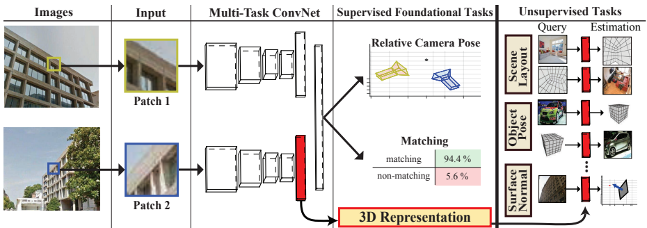
Fig.1: Learning a generic 3D representation: we develop a supervised joint framework for camera pose estimation and wide baseline matching. We then show the internal representation of this framework can be used as a 3D representation generalizable to various 3D prediction tasks.
