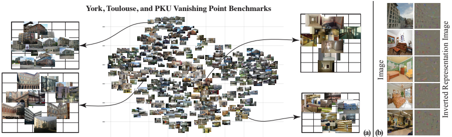
Fig. 6: a) tSNE of a superset of various vanishing point benchmarks [16,6,34] (to battle the small size of datasets). b) inversion [37] of our representation. Both plots shows traits of vanishing points.
