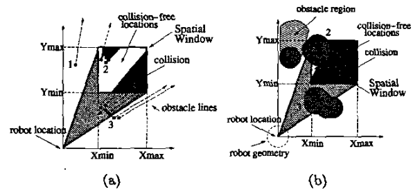
Figure 4: a) Spatial Window in the workspace. b) Spatial Window in the configuration space.
