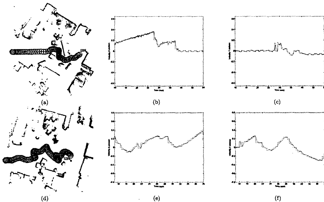
Figure 7: a,b,c) Experiment with ND and velocity profiles. d,e,f) Experiment with PFM and velocity profiles. The velocity profiles depict the computed and real robot velocities.
