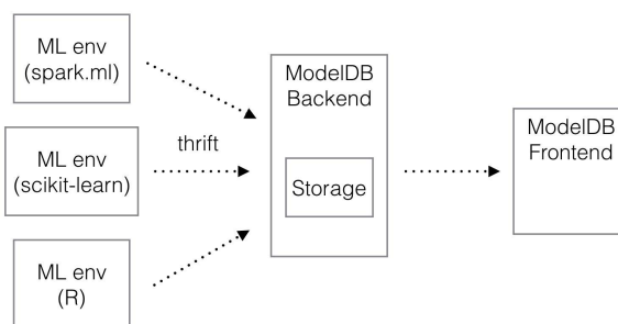
Figure 1: ModelDB Architecture
