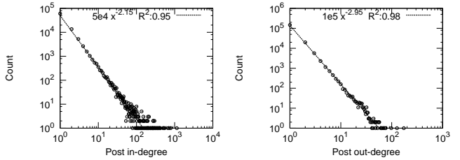
Figure 8: Post network in- and out-degree distribution.
