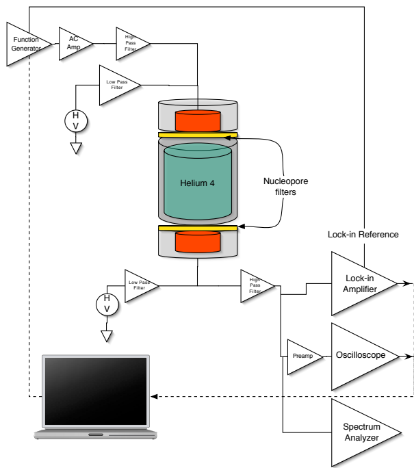
FIG. 3: Diagram of electronics and experimental setup for a frequency sweep using the “lock-in” amplifier.
